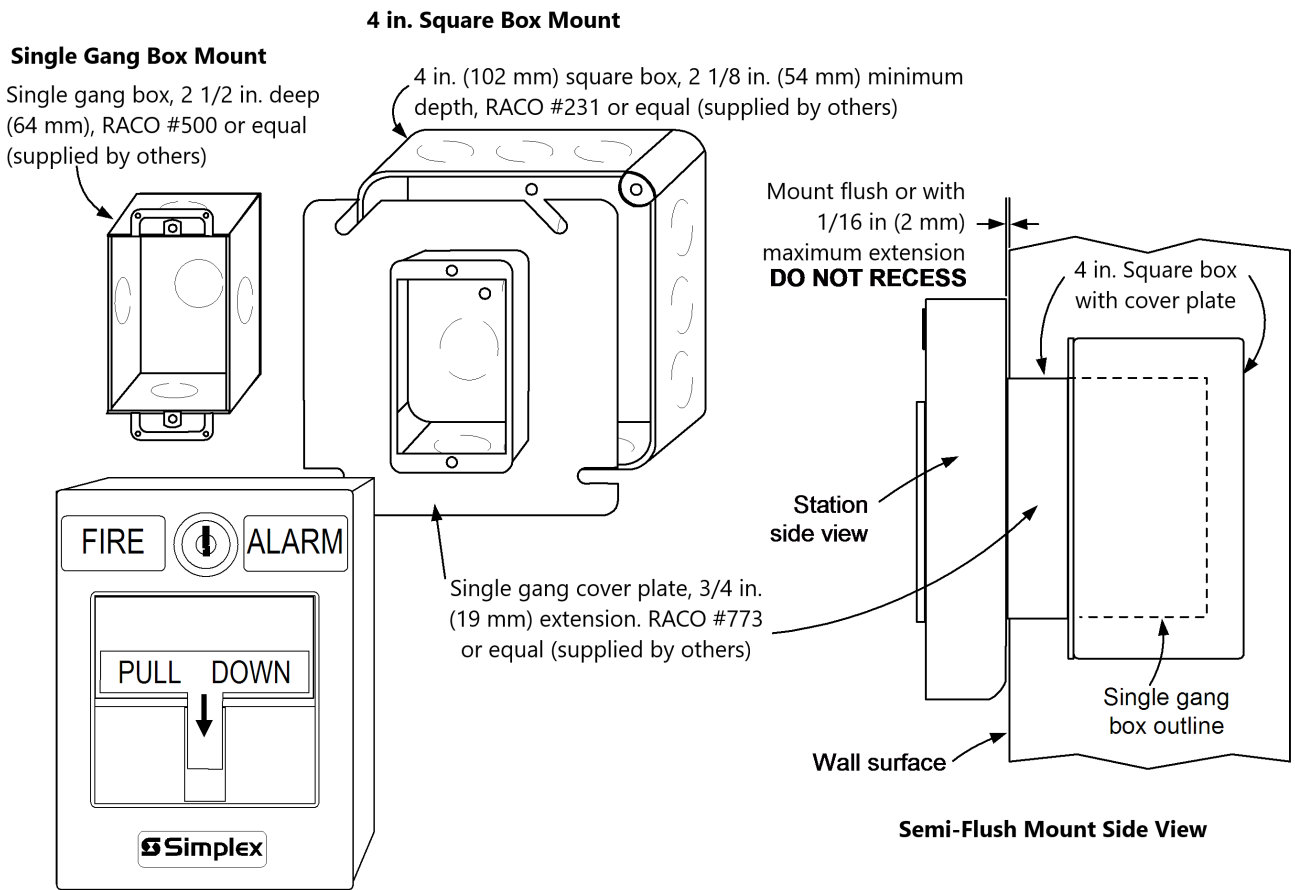
Figure 8: Semi-flush mounting reference
